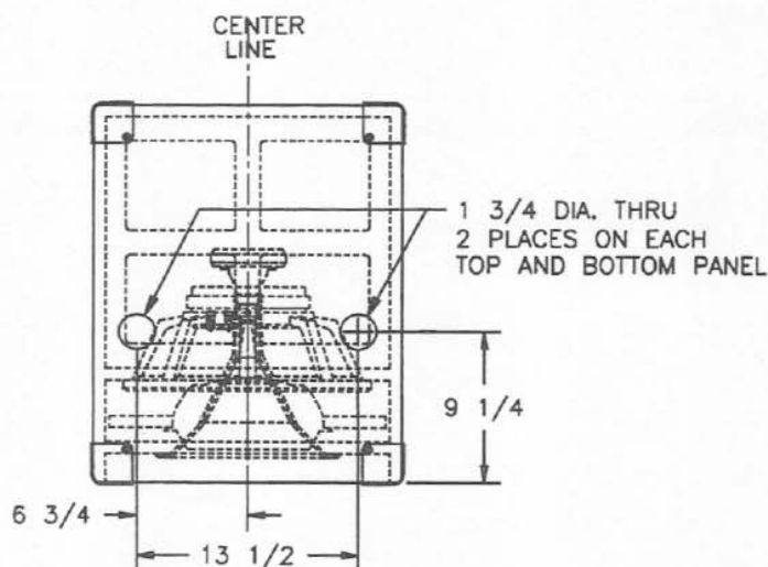
Figure 2—Drilling guide for T351
